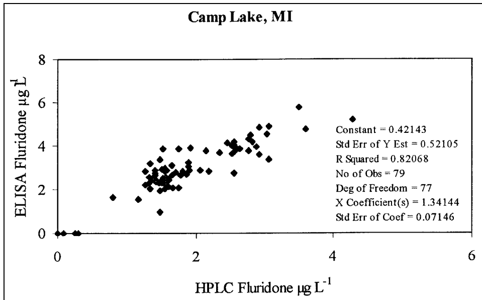
Figure 15. Comparison of ELISA and HPLC analytical methods for fluridone residues in water, Camp Lake, Michigan, 1997
