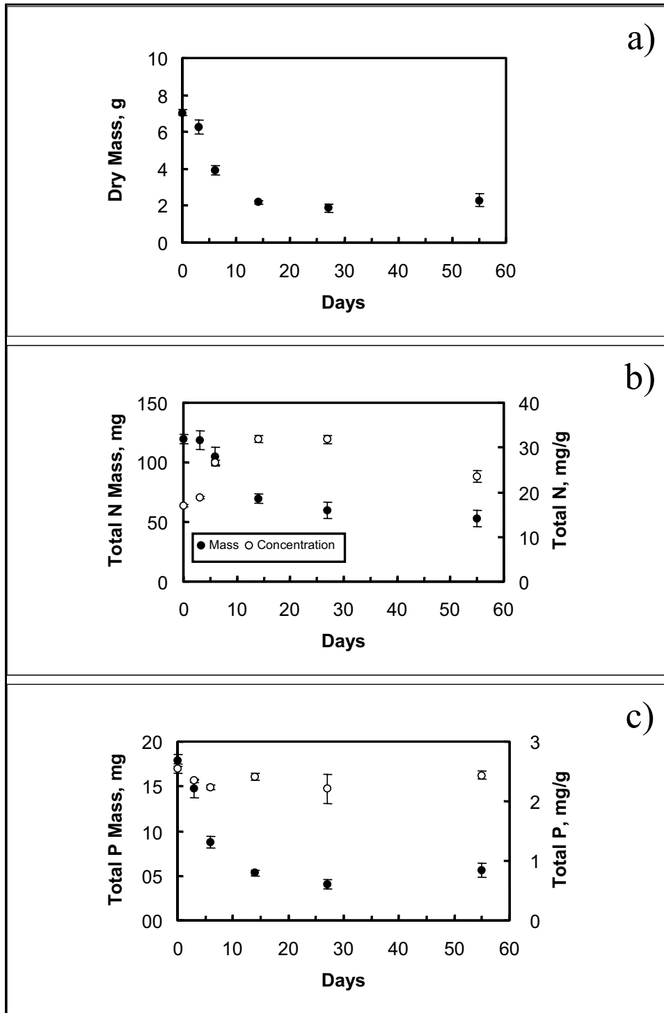
Figure 7. Waterchestnut decomposition mesh bag experiments: (a) Loss of dry mass, (b) loss of tissue nitrogen (N), (c) loss of tissue phosphorus (P) as a function of time (from James, Barko, and Eakin 2000)
