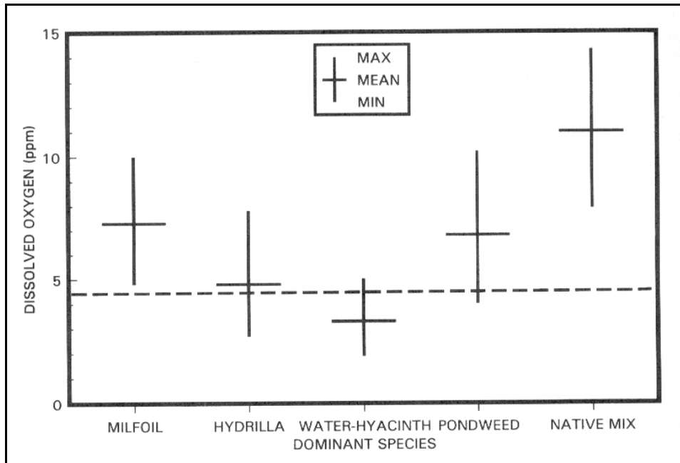
Figure 5. Maximum, minimum, and mean daily dissolved oxygen concentrations over a 48-day period in replicate ponds planted with milfoil, hydrilla, water hyacinth, floating-leaved pondweed, and a mixed native submersed plant community (from Madsen 1997)
